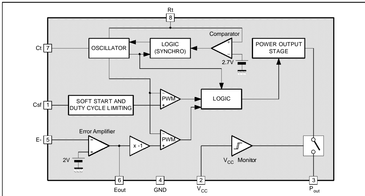
Figure 5 : Block Diagram
